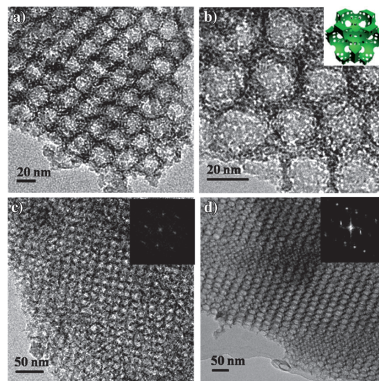
Figure 1. TEM images taken along the [110] (a, b), [100] (c), and [211] (d) directions of ODMS-C 16 -550 prepared by using EO 125 -MMA 174 and C 16 TAB as the template pair. The inset in (b) is the structural model of ODMS-C 16 -550; the insets in (c) and (d) are the corresponding FFT diffractograms.
